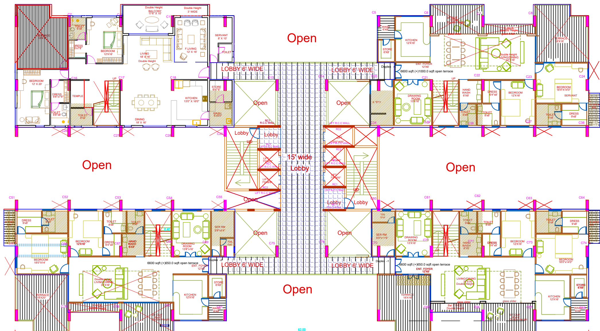
SAHIL GRAND 13 TH FLOOR PLAN changed-26 DEC 23
